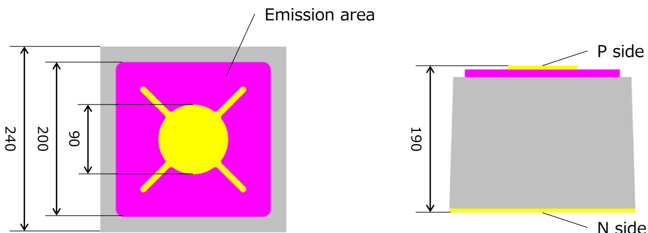
Figure 1. Electrode pattern and Chip size (Unit : μm)
